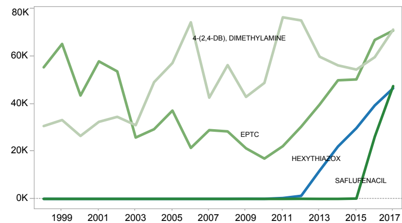
Alfalfa acres treated by the major AIs from 1998 to 2017. The graphs are ordered by the acres treated in 2017 starting with the largest amount in the upper left, moving to the right, then down. The line colors represent the AI type: blue represents insecticides, green herbicides, gray fungicides, red fumigants, insecticide/fungicides yellow, defoliant orange, and others purple. Within each graph, the lines of different AIs of one type have different color intensities
